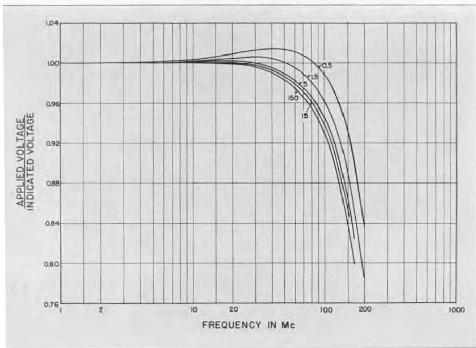
FIGURE 4. Plot of the ratio of applied voltage to indicated voltage as a function of frequency for several different levels of indicated voltage. The voltage levels are indicated by the figures associated with each curve.
