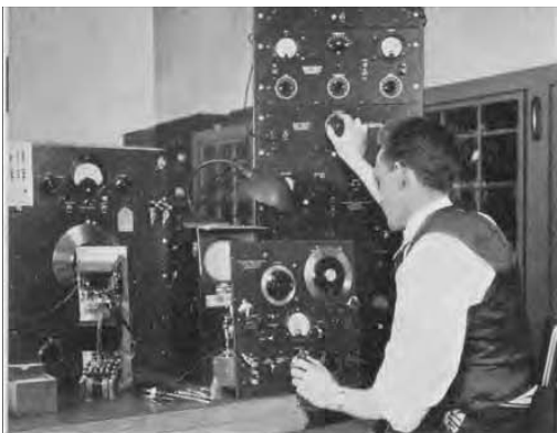
FIGURE 3. Modulation tests on a TYPE 605 Standard-Signal Generator.
