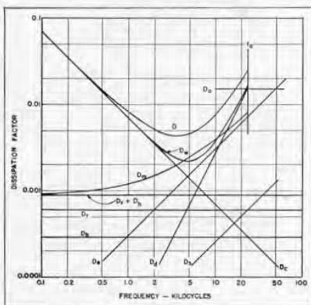
Figure 5. Evolution of the D curve for one henry toroid energized at 100 millioersteds.
