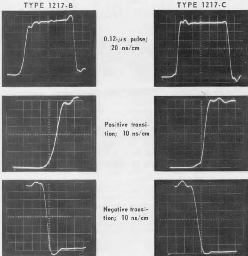
Figure 2. Oscillograms showing improvements in pulse symmetry and rise times in Type 1217-C over its predecessor.
