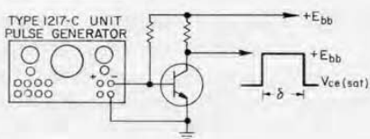
Figure 10. Control of transistor switching by Unit Pulse Generator. (top) NPN, normally on, goes off during pulse time. NPN, normally off, goes on during pulse time. PNP, normally off, goes on during pulse time. PNP, normally on, goes off during pulse time.
