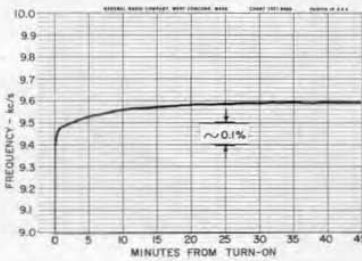
Figure 4. Warmup effects on pulse repetition frequency.
