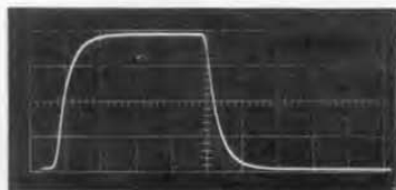
Figure 8. Oscilloscope showing effects of 12-pF probe on output pulse.
