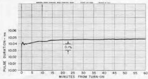
Figure 5. Warmup effects on pulse duration.
