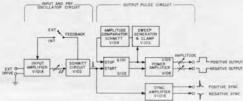
Figure 3. Block diagram.
